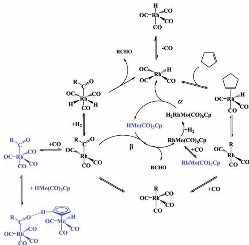
Scheme 2. Proposed Reaction Topology for Simultaneous (1) Rhodium-Catalyzed Hydroformylation, (2) Inhibition of the Rhodium Catalysis Due to the Presence of (\eta^5\text{-C}_5\text{H}_5)\text{Mo}(\text{CO})_3\text{H-C}_5\text{H}_9\text{CORh}(\text{CO})_4 , and (3) Rh–Mo CBER in Rh–Mo Bimetallic Catalysis a
