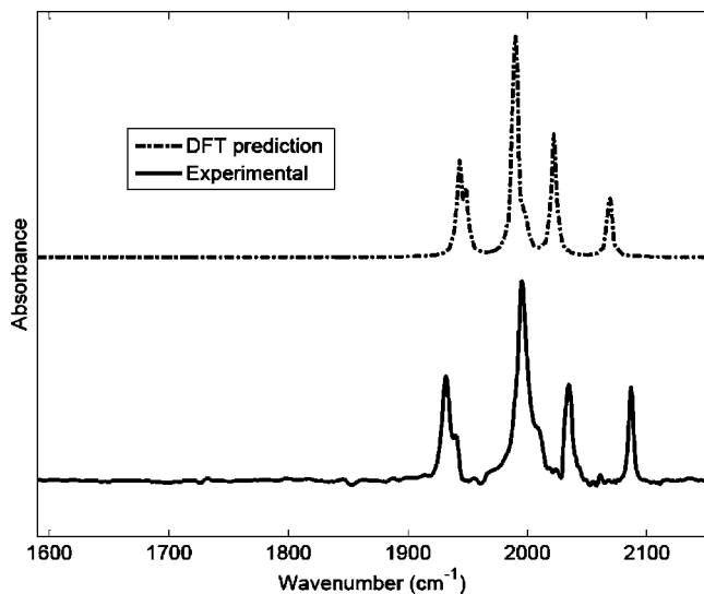
Figure 12. Comparison of the BTEM spectral estimate and DFT-predicted spectrum of (\eta^5\text{-C}_5\text{H}_5)\text{Mo}(\text{CO})_3\text{-Rh}(\text{CO})_4 .
